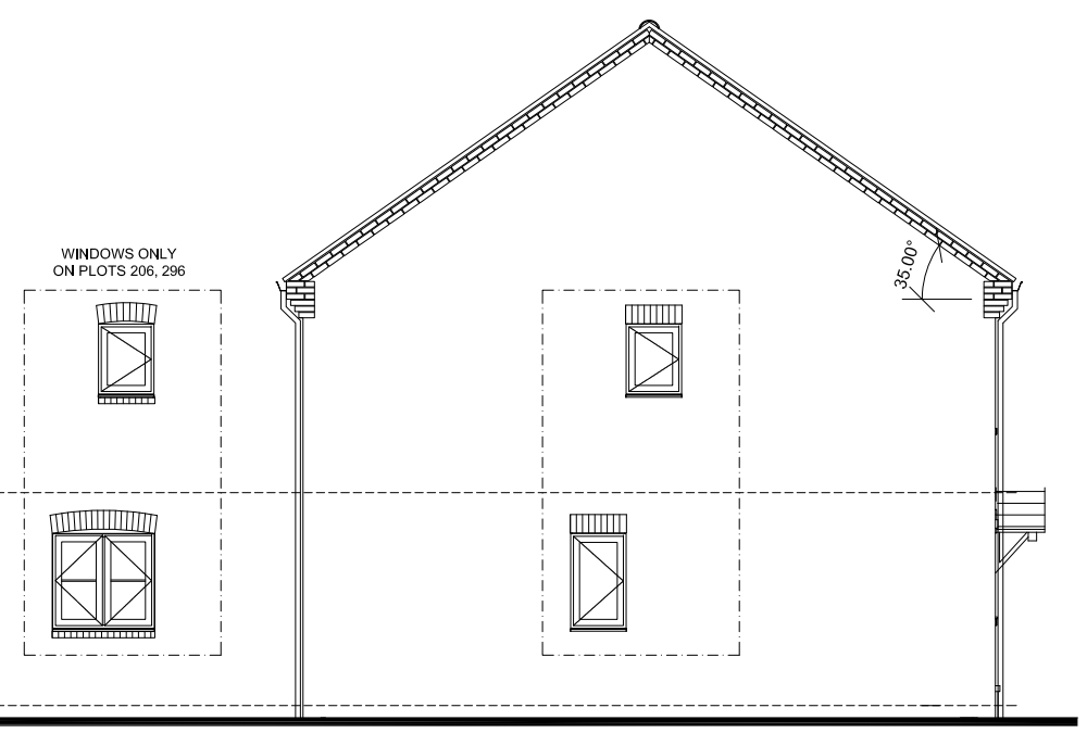
LEFT ELEVATION
